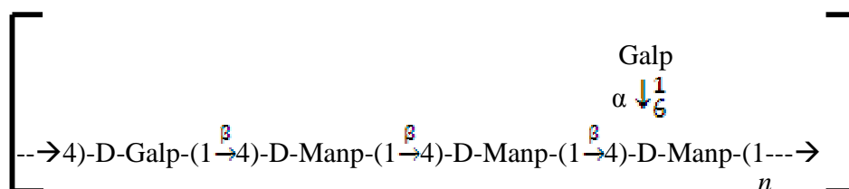
Figure : Seeds polysaccharide structure of Cassia alata Linn. plant.
